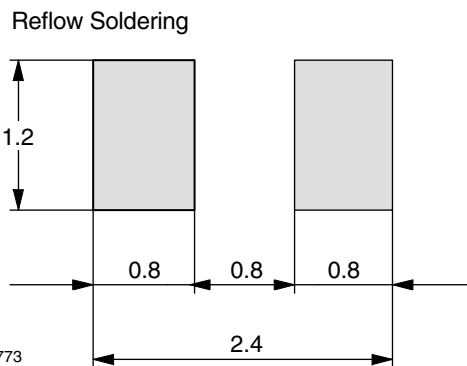
Fig. 11 - Recommended Foot Pads (in mm)
