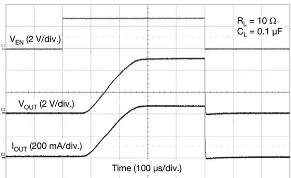
Fig. 22 - Switching (V IN = 5 V)
