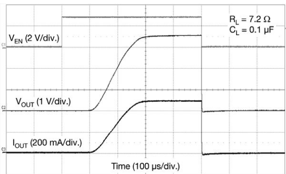
Fig. 21 - Switching (V IN = 3.6 V)
