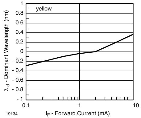
Fig. 19 - Dominant Wavelength vs. Forward Current
