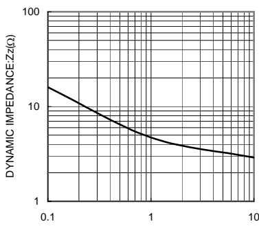
ZENER CURRENT(mA) Z_z - I_z CHARACTERISTICS
